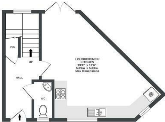
GROUND FLOOR 341 sq.ft. (31.7 sq.m.) approx.
